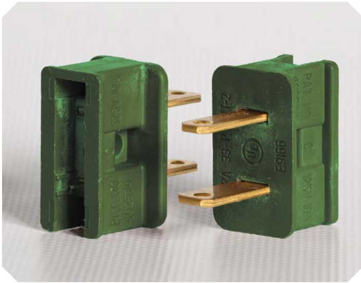
Zip Dual Male SPT1/SPT2 (covers included)
